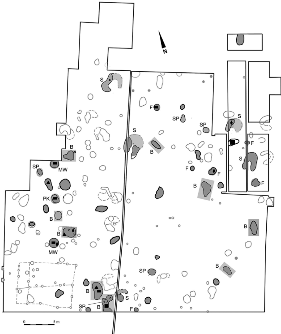
Fig. 6. Niesułowice; the younger settlement stage.
