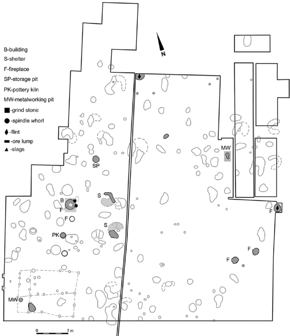
Fig. 4. Niesułowice; the older settlement stage. Ryc. 4. Niesułowice, starsza faza osadnicza.
