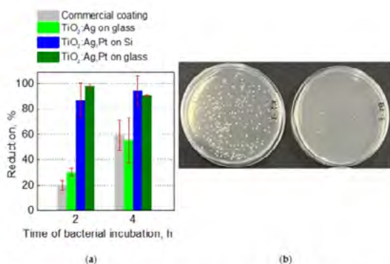
Reduction of S. aureus bacteria on coatings (a) and example dishes with bacterial colonies (b) from the control plate (left) and from the TiO 2 :Ag,Pt/Si coating (right).
